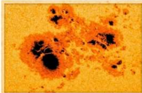
Active Region 12192, a sunspot, is likely to produce coronal mass ejections, which could wreak havoc on satellites and power grids. CREDIT: NASA/SDO/Zel
