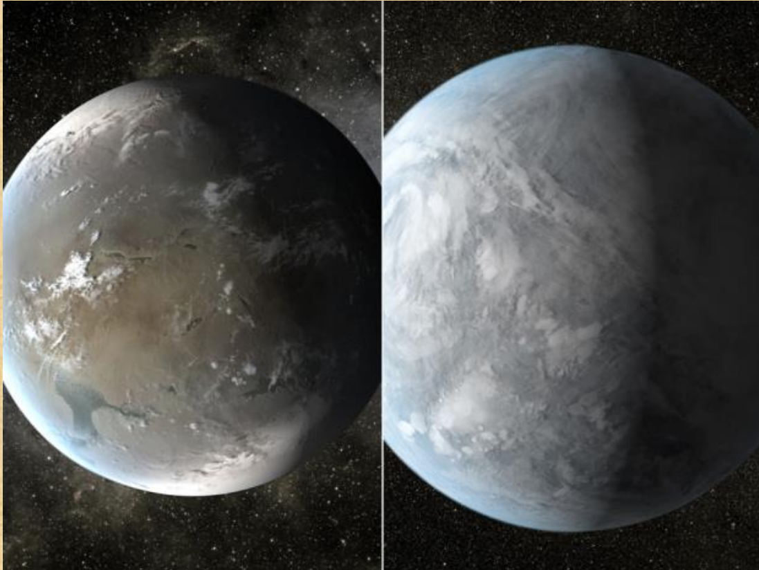
Kepler 62f, left, and Kepler 62e, right
